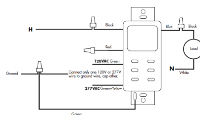
WIRING DIAGRAM: THREE-WAY INSTALLATION SS700Z
